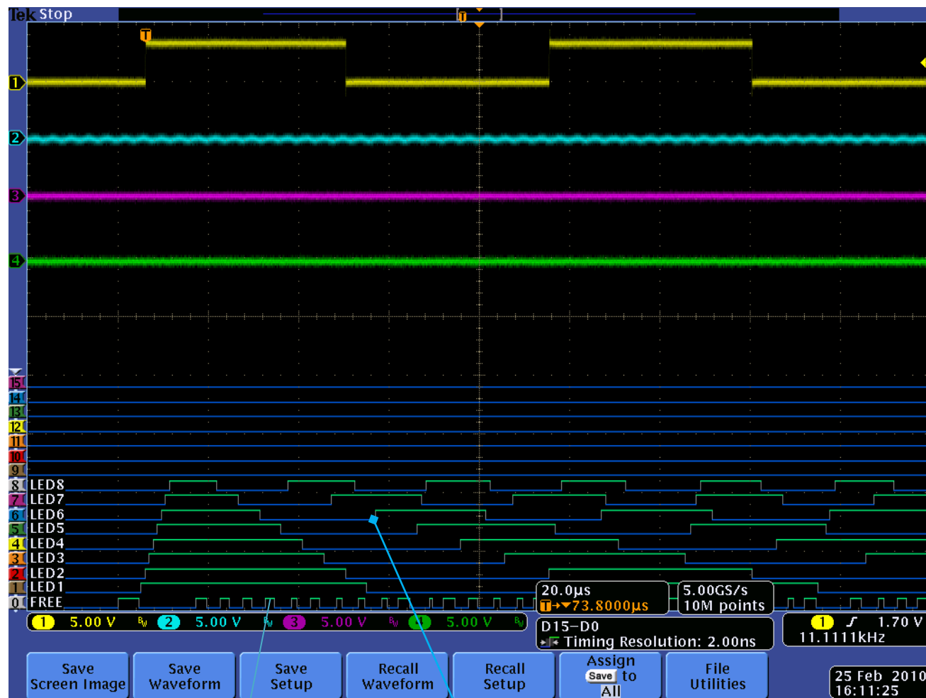
Oscilloscope screen shot of Free Time indicator plus 8 simultaneous LED pulsers operating at different rates.
